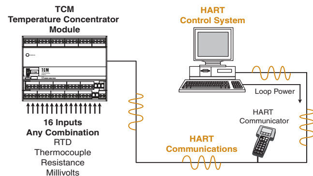
Figure 2. TCS in general purpose or Class I, Division 2 or Zone 2 HART Communications Mode (accommodates one TCM per system).
